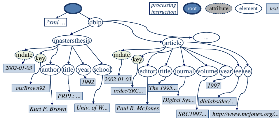
Figure 11.2: Example data model representation for the XML fragment of Figure 11.1. Note that the different node types are represented here using different shapes.
