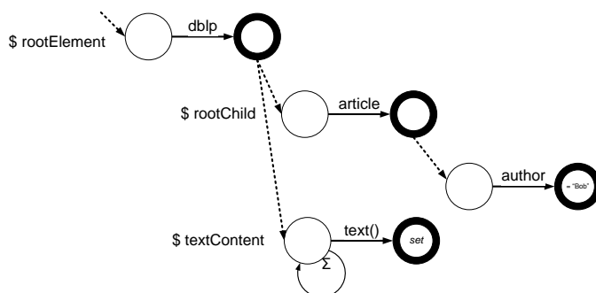
Figure 11.8: Hierarchy of nondeterministic finite automata for matching the set of XPath expressions in the XQuery of Figure 11.5. Note that upon reaching the final state of one machine, we may activate other (nested) XPath expressions, and we may need to test the match against a value or collect it within a set.
