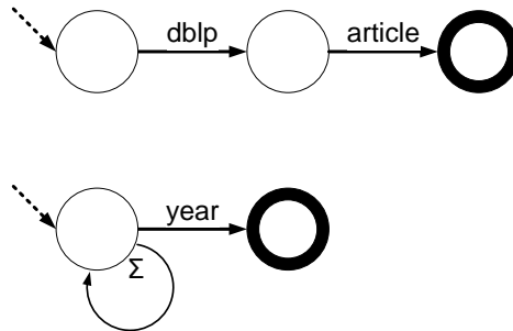
Figure 11.7: Nondeterministic finite automata for the XPath expressions /dblp/article and //year . Note that the \Sigma on the edge label in the automata represents the alphabet of all possible labels, i.e., a wildcard.
