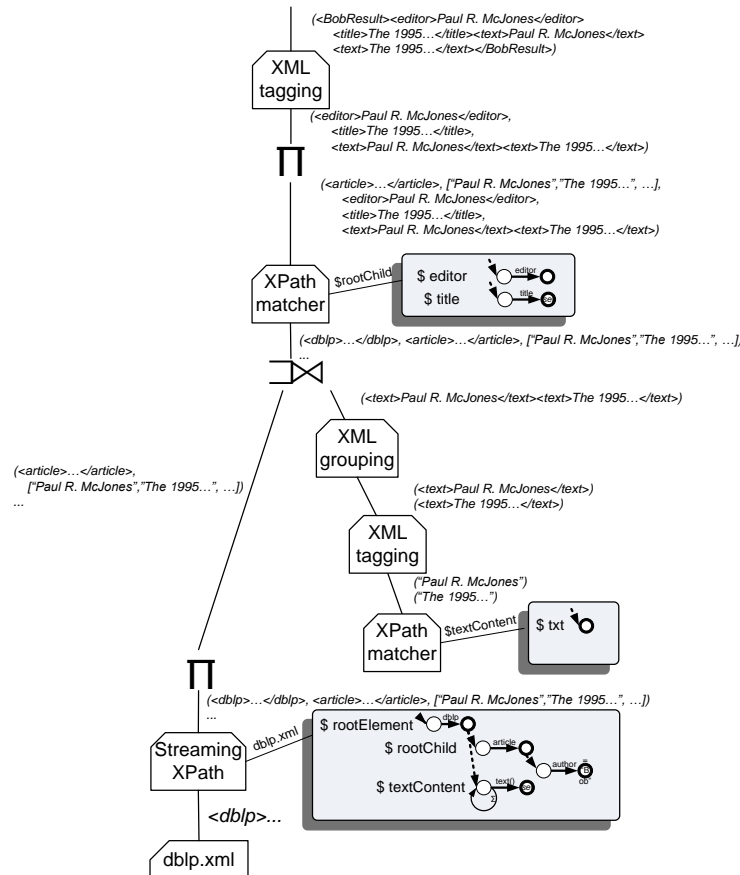
Figure 11.6: Sketch of a query plan for the query of Figure 11.5. Most of the engine remains a tuple processor, where tuples are no longer in first-normal-form, but rather binding tuples containing (references to) trees.
