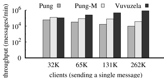
FIGURE 9—Pung’s multi-retrieval optimizations increase its throughput by up to 5.2\times . Pung-M represents a version of Pung where clients retrieve k=64 messages simultaneously using our hybrid scheme (§4.4). At 262K clients, Vuvuzela handles 84.9\times and 22.6\times more messages than Pung and Pung-M, respectively.
