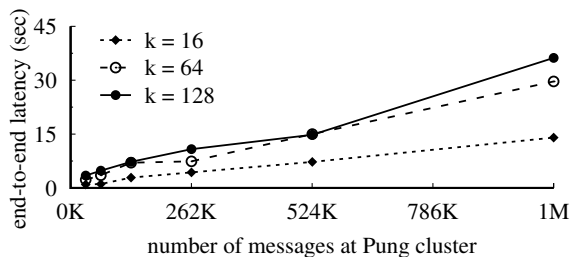
FIGURE 8—The end-to-end latency of sending one message and retrieving k using Pung’s multi-retrieval. It takes 36.2 seconds with k = 128 and 1M tuples. This is 4.6\times faster than retrieving 128 messages using Pung’s single-retrieval (Fig. 6).
