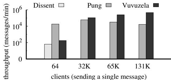
FIGURE 7—Pung can handle significantly more messages and clients than Dissent but its throughput at 131K clients is 27.8\times lower than Vuvuzela’s. We do not report Dissent’s throughput past 64 users (see text for details).
