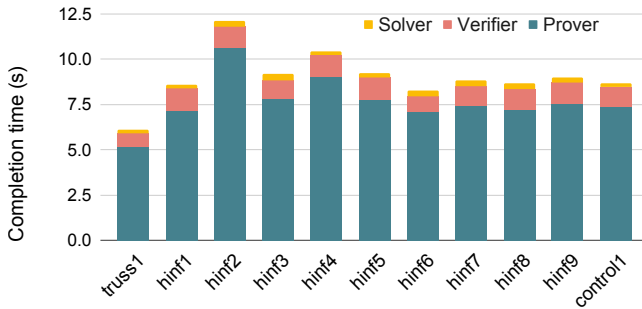
FIGURE 9—Runtime attribution of SDP benchmarks in Otti.
