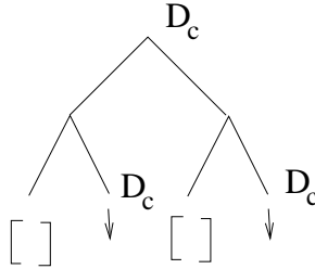
Figure 2. An initial tree for parallel constructions. [] stands for the feature structure that anchors the tree and which can be realised by any lexical item with a compatible feature structure.
