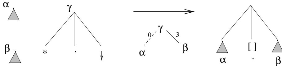
Figure 4. TAG derivation of Example 5
