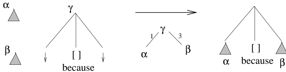
Figure 6. TAG derivation of Example 11
