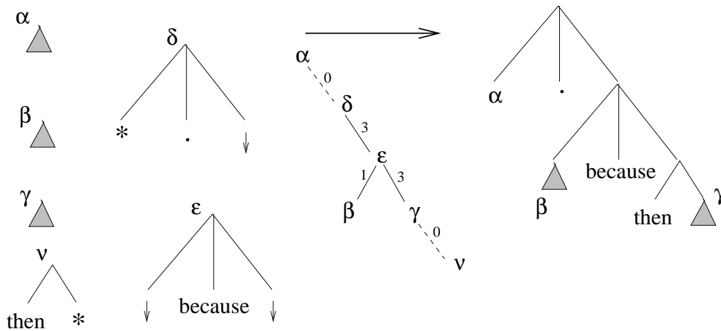
Figure 7. TAG derivation of Example 22
