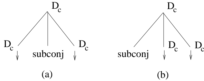
Figure 1. Initial trees (a-b) for a subordinate conjunction. Here, D_c stands for “discourse clause”, \downarrow indicates a substitution site, while “subconj” stands for the particular subordinate conjunction that anchors the tree.
