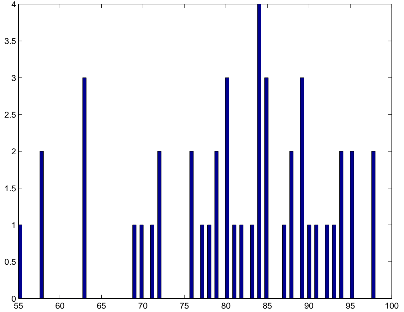
HW1 score distribution: N = 46, mean = 81, median = 83.5, max = 98, min = 55
