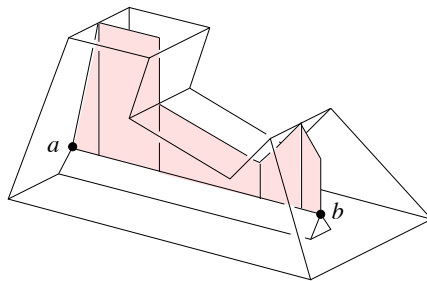
Fig. 49. The fence of the segment ab consists of five walls, each a triangle or a quadrangle
