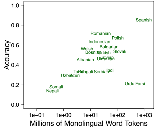
Figure 4: Millions of monolingual word tokens vs. Lexicon Induction Top-10 Accuracy
