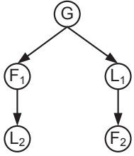
Figure 6: Fork and Loop Hierarchy T_G
