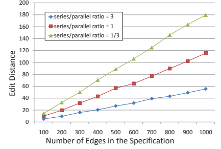
Fig. 12. Series vs Parallel (edit distance)
