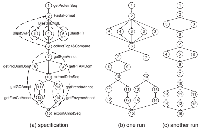
Fig. 1. Protein annotation workflow specification and runs
