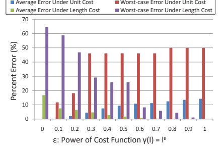
Fig. 15. Varying cost models
