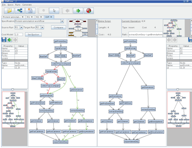
Fig. 9. PDiffView snapshot
