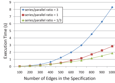
Fig. 11. Series vs Parallel (execution time)
