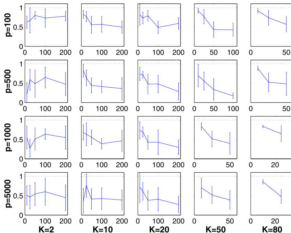
Fig. 5 Average of the ratio of the number of active covariates for Algorithm 1 and the same quantity for the TY algorithm. These ratios are based on five replicates, and one standard deviation confidence intervals are indicated. The models selected by Algorithm 1 are almost always sparser than those returned by the TY algorithm
