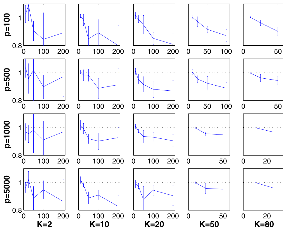
Fig. 4 Average of the ratio of the error rate on the test set for Algorithm 1 and the TY algorithm. These ratios are based on five replicates, and one standard deviation confidence intervals are indicated. Note that the average error rate of Algorithm 1 is almost always smaller than that of the TY algorithm. The improvement in error rate is typically significant for larger number of tasks and larger ambient dimension
