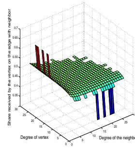
Figure 6: Edge division versus edge endpoint degrees in NBS for PA(50, 3)
