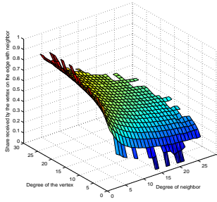
Figure 5: Edge division versus edge endpoint degrees in PBS for PA(50, 3)
