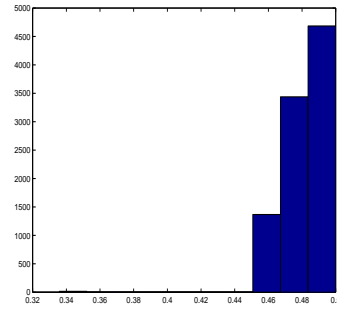
Figure 4: A histogram of NBS for division on each edge, for PA(50, 2)
