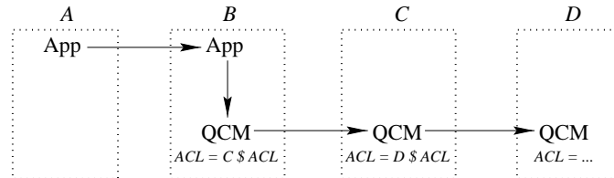
Figure 3. Pushing and Pulling Certificates
