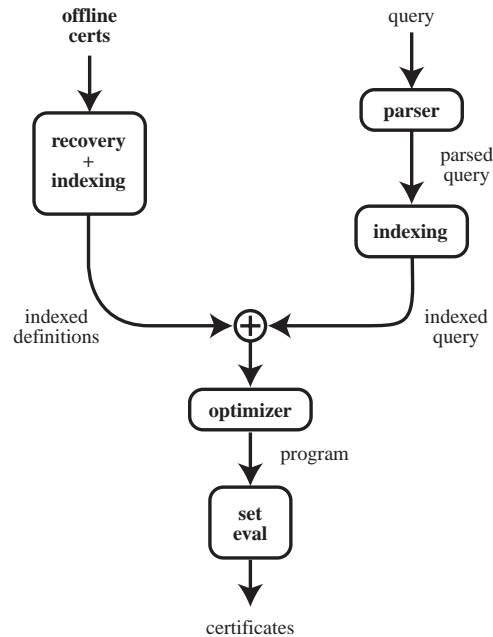
Figure 7. Offline QCM evaluation
