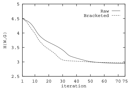
Figure 2: Convergence for the ATIS Corpus
