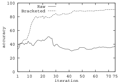
Figure 3: Bracketing Accuracy for the ATIS Corpus
