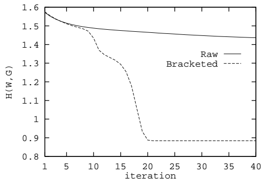
Figure 1: Convergence for the Palindrome Corpus
