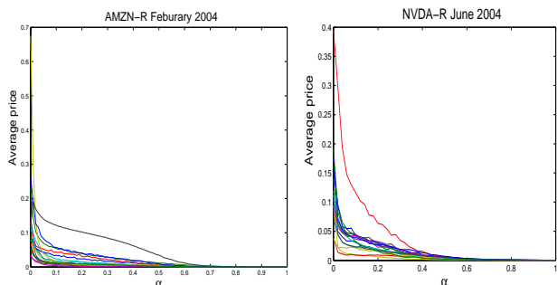
Figure 5: Percentage change to the average execution price (y-axis) vs. probability of treating arriving INET orders as absolute prices (x-axis). The left panel is for AMZN, the right panel is for NVDA, and each curve corresponds to a single day of trading during a month of 2004. Curves represent averages over 1000 trials.
