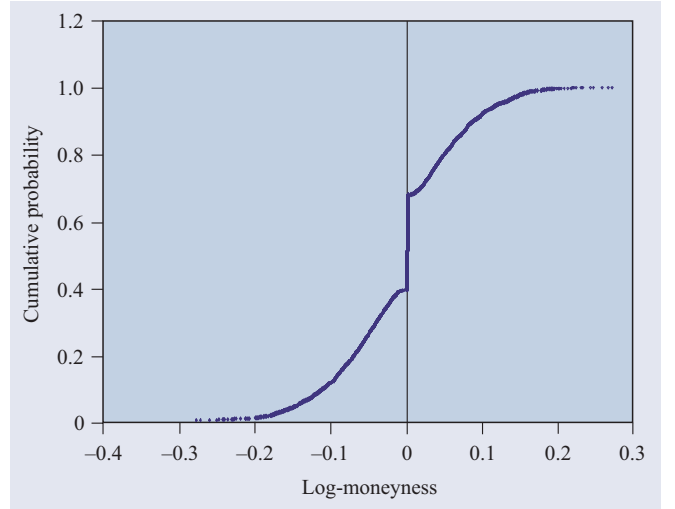
Figure 6. Cumulative probability distribution function computed by Monte Carlo simulation. The step corresponds to the fact that a finite fraction of the paths is pinned at the strike.
