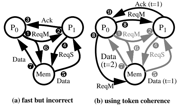
Figure 2. Example Race. A request for shared (ReqS) racing with a request for modified (ReqM).
