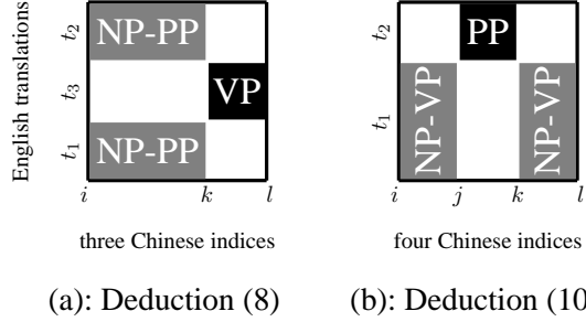
Figure 3: Illustrations of two deductions with gaps.
