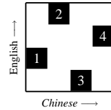
Figure 2: An example of non-binarizable rule from the hand-aligned Chinese-English data in Liu et al. (2005). The SCFG rule is VP \rightarrow ADVP^{[1]} PP^{[2]} VB^{[3]} NN^{[4]} , VP \rightarrow VB^{[3]} JJ^{[1]} NNS^{[2]} PP^{[2]} in the notation of Satta and Peserico (2005).
