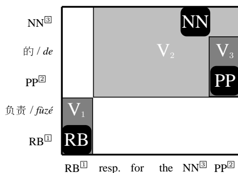
Figure 11 Alignment matrix of the SCFG rule (6). Areas shaded in gray and light gray denote virtual nonterminals (see rules in (7)).
