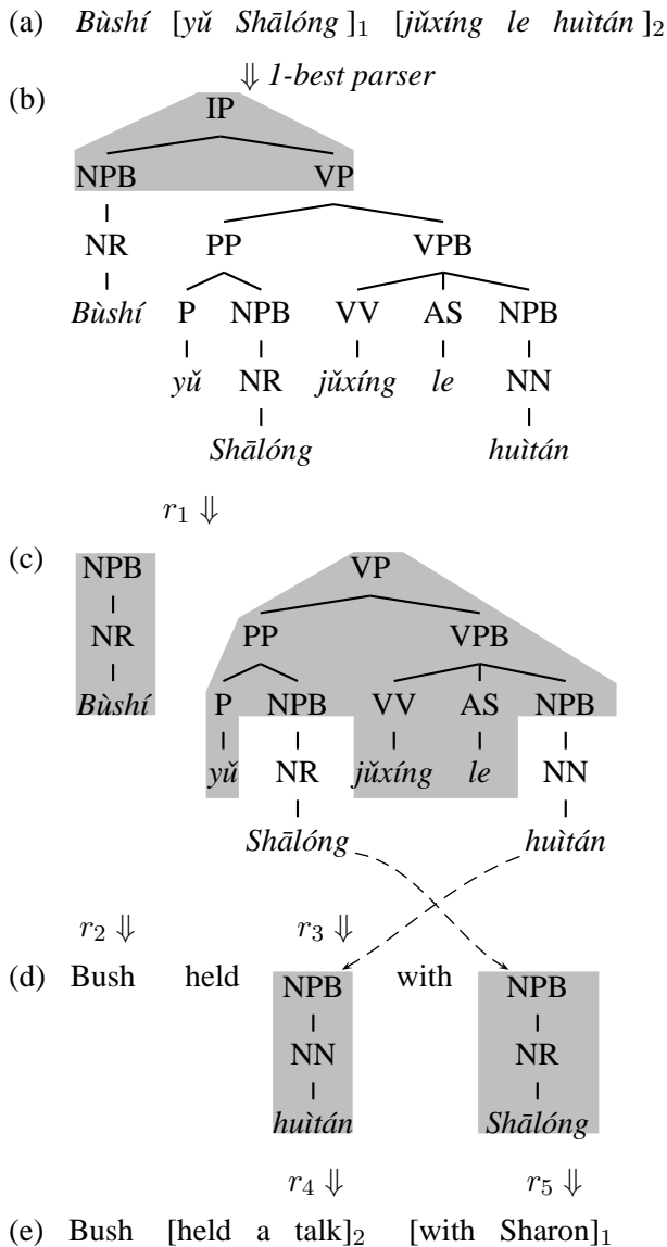
Figure 2: An example derivation of tree-to-string translation. Shaded regions denote parts of the tree that is pattern-matched with the rule being applied.
