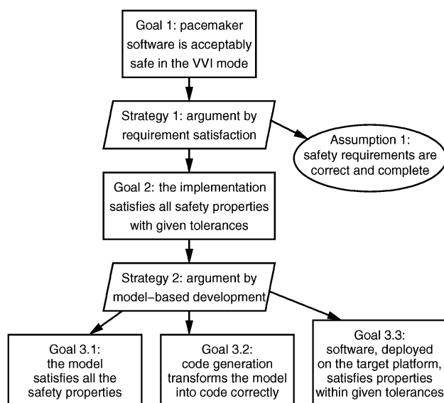
Fig. 8. Top-level claims of the pacemaker assurance case.
