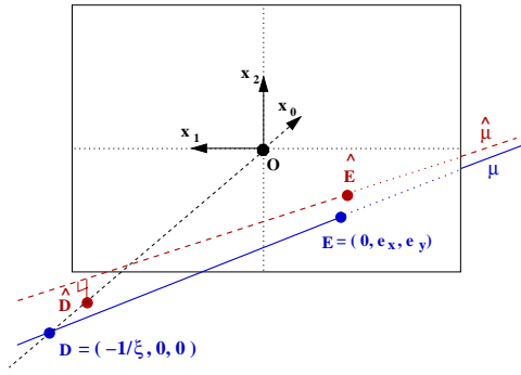
Figure 2: Line \mu represents the left/right null space of \mathbf{F} . The line goes through points \mathbf{E} and \mathbf{D} . The former encodes the epipole on the undistorted image plane and the latter encodes the distortion parameter
