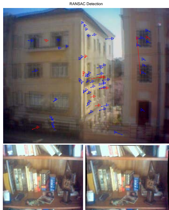
Figure 6: Estimation of the Radial Fundamental Matrix in images acquired with a Sony-Ericsson cell phone. The quality of the 288 \times 352 images was significantly worse when compared with images used in the previous examples. In order to compute the fundamental matrix we used a modified version of the 15-point algorithm that assumes that the radial distortion of the two views is the same. We also increased the threshold for the detection of inliers. The Lowe detector found 68 correspondences from which 59 were considered inliers. The distortion estimation was 19 pixels. This value was used to correct the bottom image
