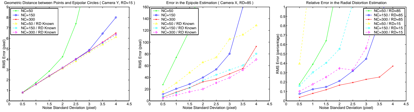
Figure 3: Tests on synthetic data. The synthetic image size is 480 \times 640 and the radial distortion on the two views is different. The distortion in camera X causes a deviation of 85 pixels at the image corner while in camera Y the shift along the radial direction is only 15 pixels. The graphics show the performance of the 15-point algorithm in estimating the radial fundamental matrix from 50, 150 and 300 correspondences. The robustness to noise clearly improves with the number of correspondences (NC). For an increasing NC the performances of the 15-point and 8-point algorithms seem to converge.
