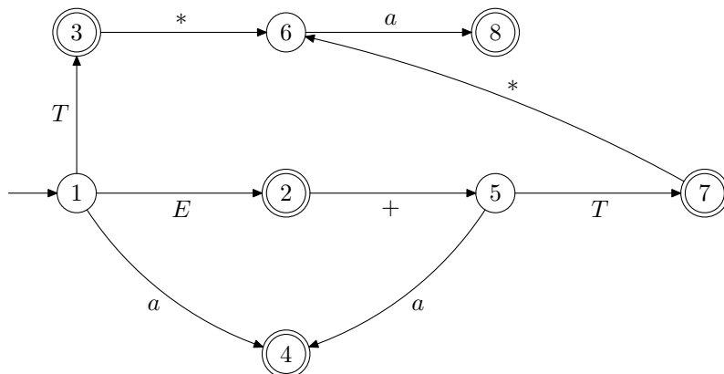
Figure 7.5: DFA for C_{G_2}
