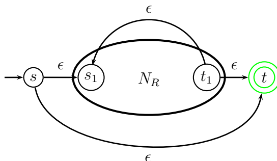
Figure 5.9: NFA for R^*
