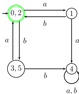
Figure 5.19: A minimal DFA D_2 for L = \{ab, ba\}^*
