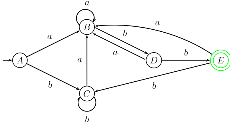
Figure 5.17: A non-minimal DFA for \{a, b\}^*\{abb\}
