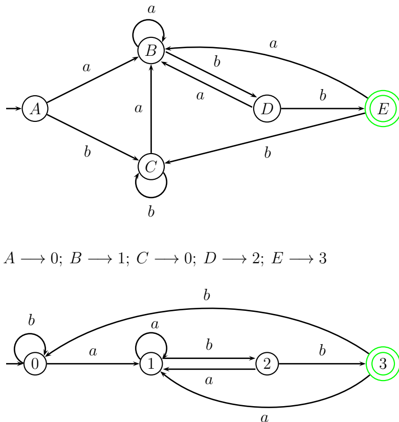
Figure 5.1: A map of DFA's
