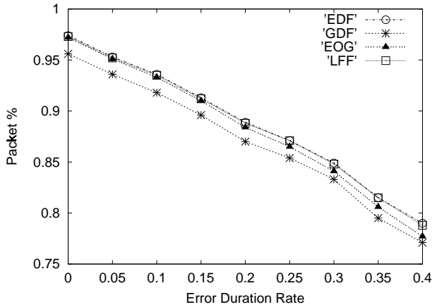
Figure 2. System Throughput (\frac{\sum_{i=1}^N M_i^a}{\sum_{i=1}^N M_i})
