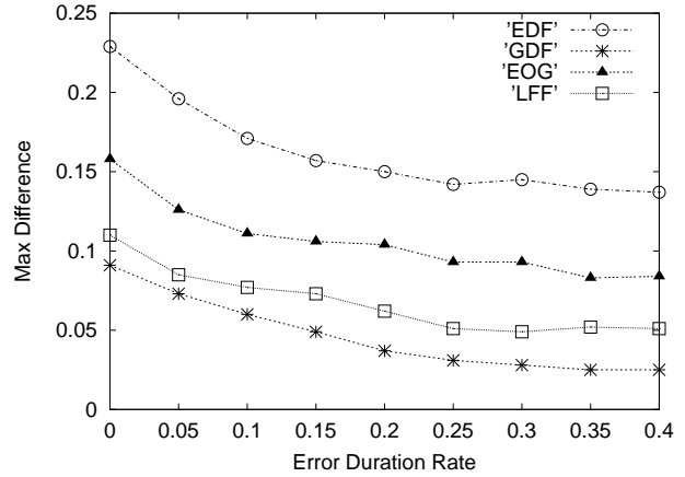
Figure 4. Maximum of |\epsilon_i - \epsilon_j|
