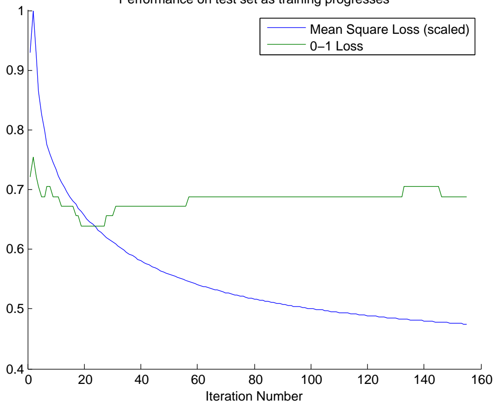
Performance on test set as training progresses
