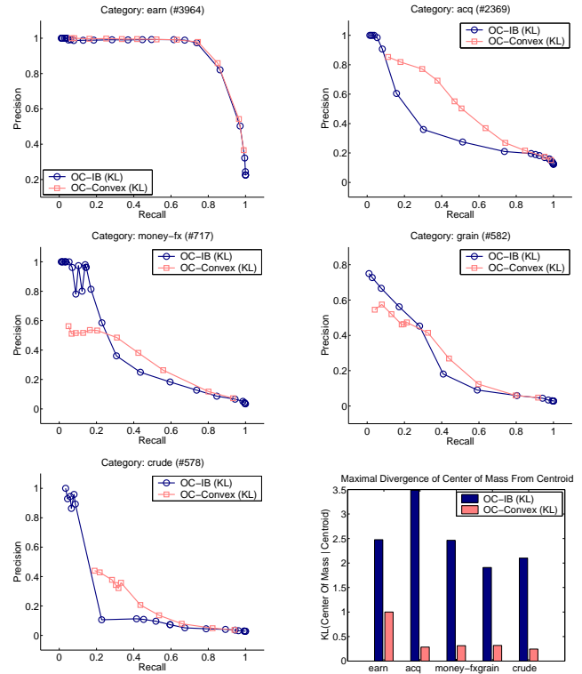
Figure 5. Plot of Precision vs. Recall for the five topics of Reuters-21578. Two algorithms are compared: one-class IB (OC-IB). The number near the category in the title indicates the total number of examples associated with this category. Right-bottom-figure: plot of the maximal distance of the resulting centroid and the center of mass of the training set. The maximum is taken for each of the algorithms over the possible values of tuning parameters.
