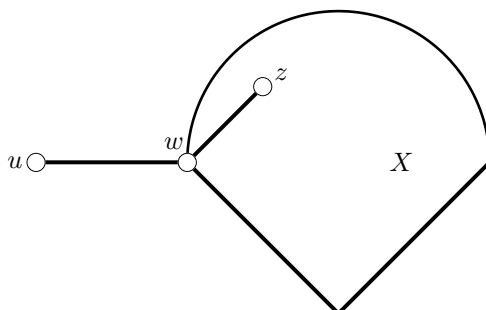
Figure 26.2: Inequality of Lemma 26.1.5
