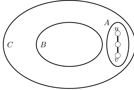
Figure 26.1: Inequality of Lemma 26.1.3
