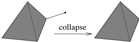
Figure 8: Collapsing a vertex together with the only edge that contains it.
