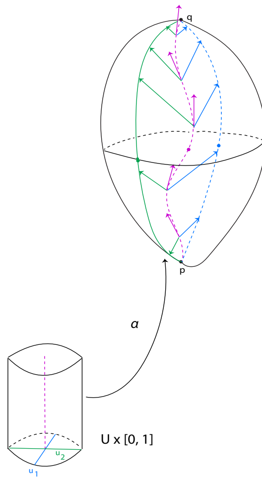
Figure 14.1: A 2-parameter variation \alpha . The pink curve with its associated velocity field is \alpha(0, 0, t) = \gamma(t) . The blue vector field is W_1(t) while the green vector field is W_2(t) .
