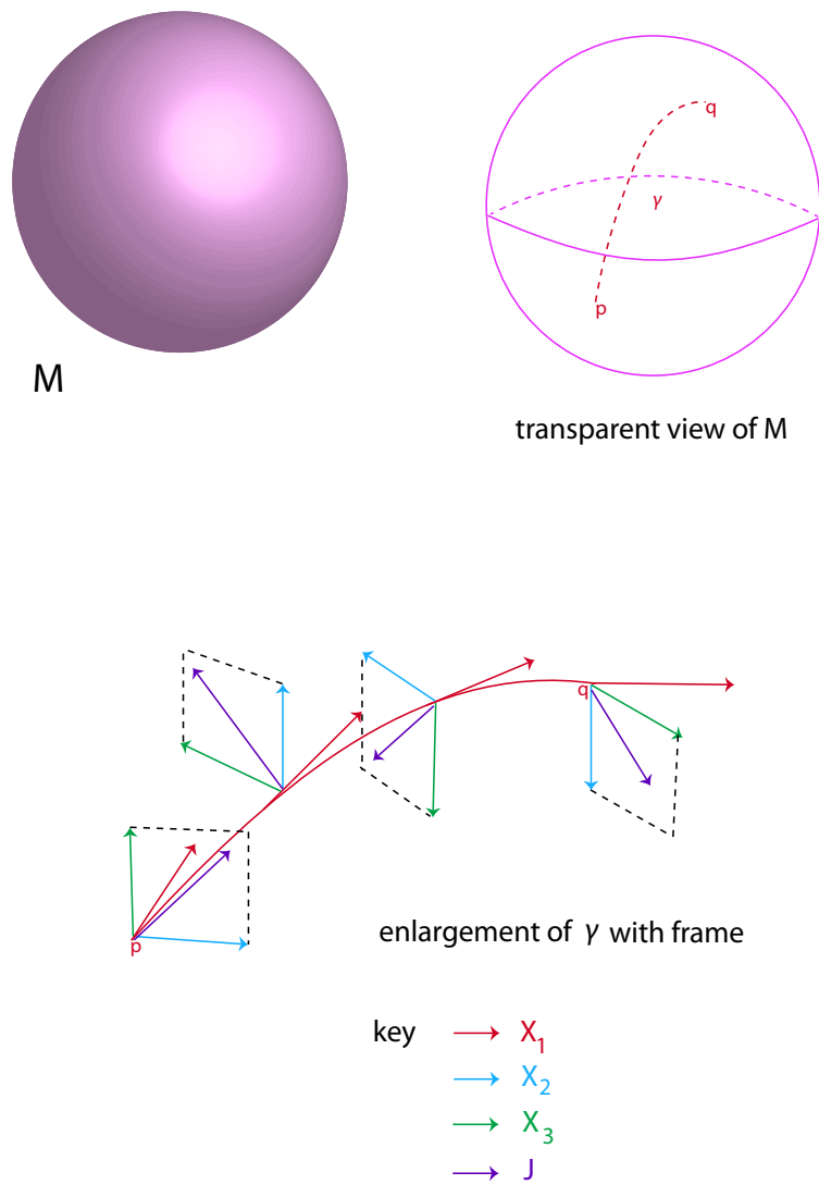
Figure 14.2: An orthogonal Jacobi field J for a three dimensional manifold M . Note that J is in the plane spanned by X_2 and X_3 , while X_1 is in the direction of the velocity field.
