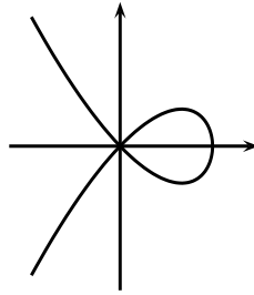
Figure 5.1: A nodal cubic; not a manifold
