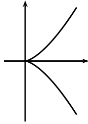
Figure 5.2: A Cuspidal Cubic
