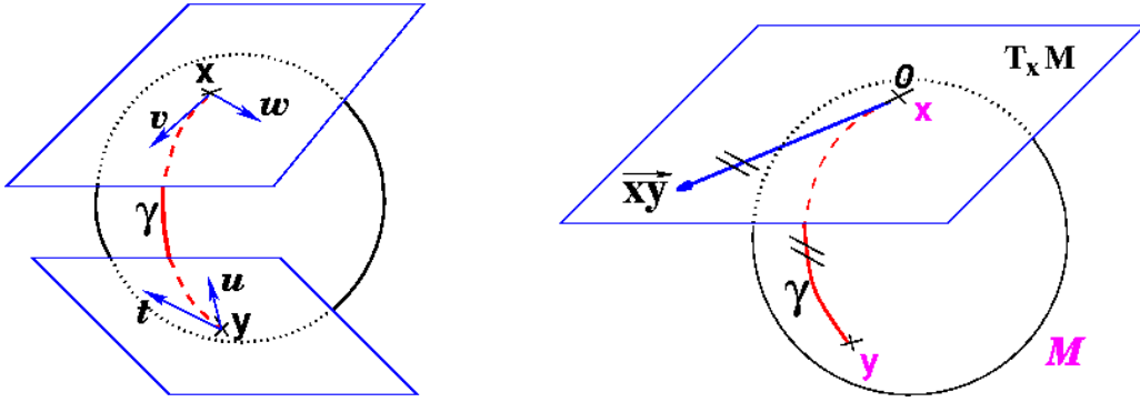
Figure 1: Left: The tangent planes at points x and y of the sphere \mathcal{S}_2 are different: the vectors v and w of T_x \mathcal{M} cannot be compared to the vectors t and u of T_y \mathcal{M} . Thus, it is natural to define the scalar product on each tangent plane. Right: The geodesics starting at x are straight lines in the exponential map and the distance along them is conserved.
