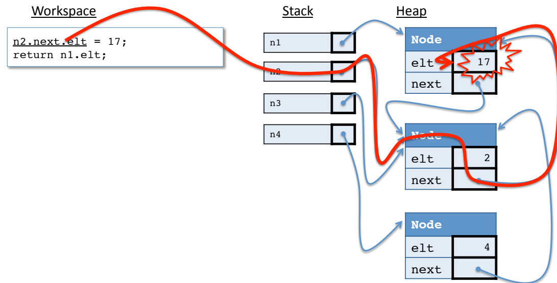
Figure 22.7: After a few more steps, the final update.
