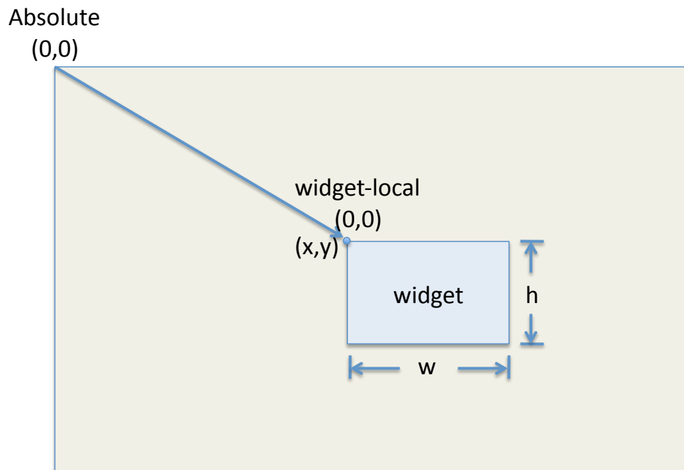
Figure 18.2: A widget draws itself in terms of widget-local coordinates, which are made relative to the global coordinate system by using a Gctx.t value, which, among other things, contains the (x,y) “offset” from the origin of the graphics window. Here the grey region represents the entire graphics window. Each widget also keeps track of its width and height, which are needed for computing layout information.
