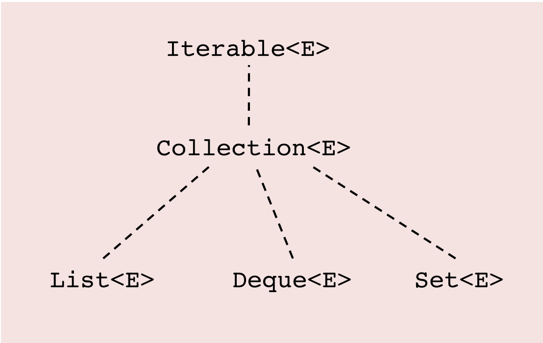
Figure 25.4: The iterable interface.
