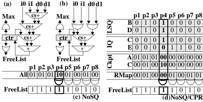
Figure 4. Binary and hybrid reference counting mechanisms.
