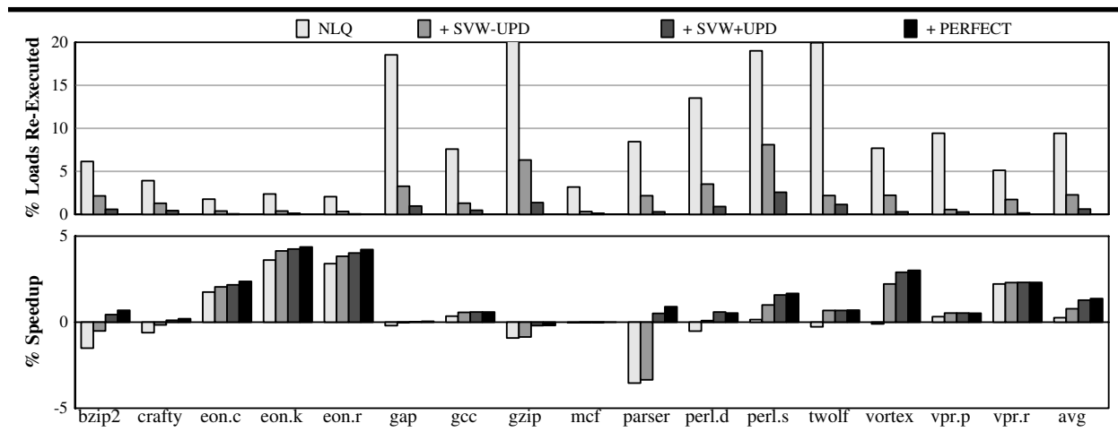
FIGURE 5. NLQ LS re-execution rate (top) and performance (bottom).
