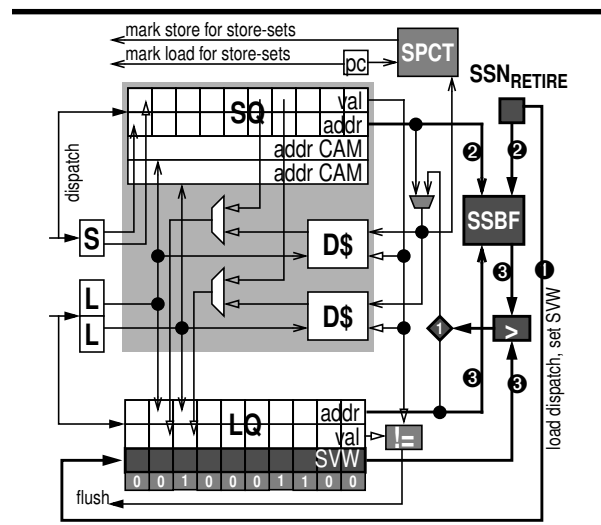
FIGURE 3. NLQ with SVW.
