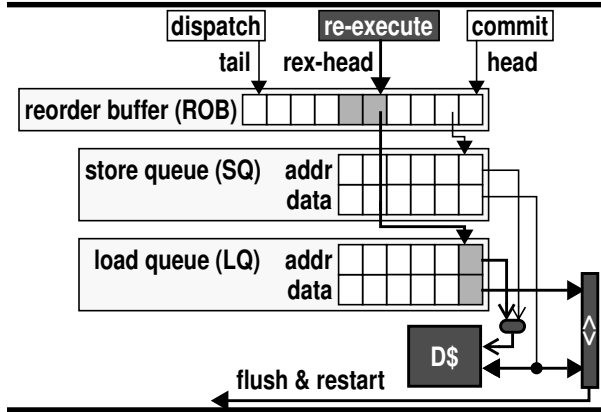
FIGURE 1. Pipeline with load re-execution engine. Re-execution shares a data cache port with store retirement.
