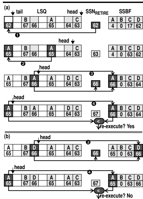
FIGURE 4. NLQ LS +SVW working example shows the relevant SVW steps in the life of one dynamic load, the one on the left-most side of the LSQ. In (a), the steps are load dispatch, load execution, conflicting store retirement/SSBF update, and load SSBF lookup/re-execution. (b) shows alternatives for the last two steps.
