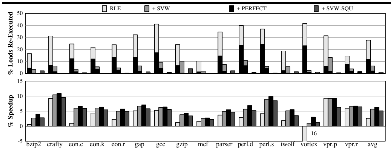
FIGURE 7. RLE re-execution rate (top) and performance (bottom).
