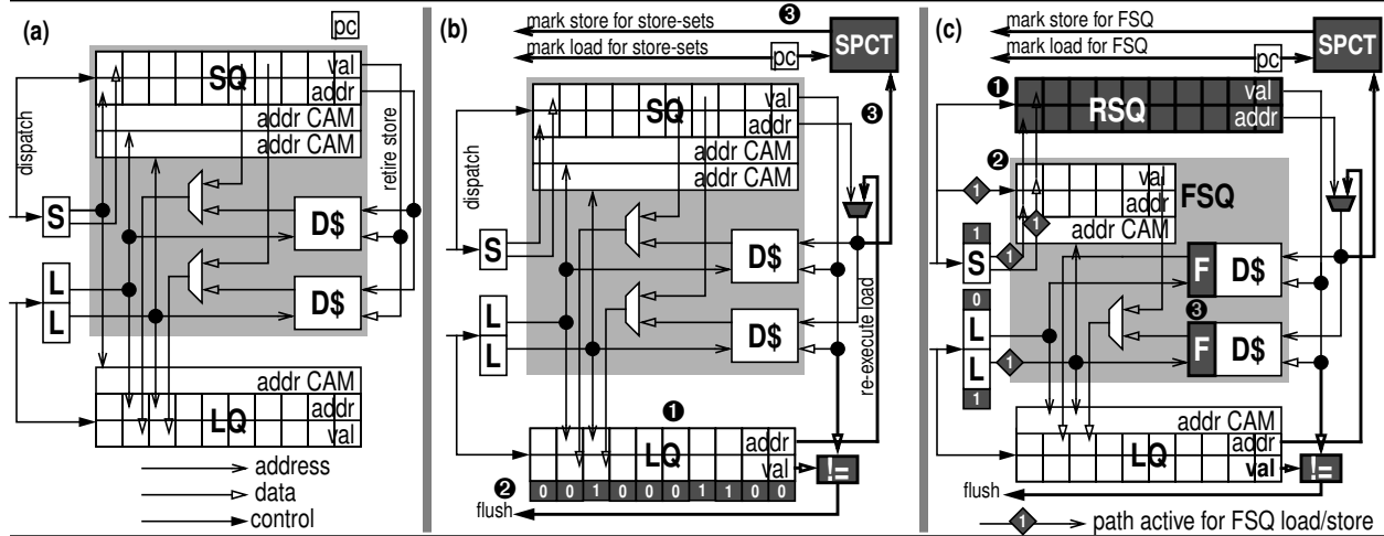
FIGURE 2. LEFT: conventional load-store unit with interleaved data cache, two load ports and one store port. MIDDLE: non-associative LQ design replaces LQ searches with re-execution. RIGHT: speculative SQ design splits SQ into a small, low-bandwidth forwarding queue (FSQ) and large non-associative retirement queue (RSQ). Re-execution checks that loads and stores are correctly steered to the FSQ. Steering is performed by a predictor which is trained by re-execution mechanism.
