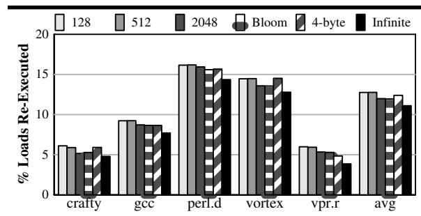
FIGURE 8. SSBF organization and re-execution rate.
