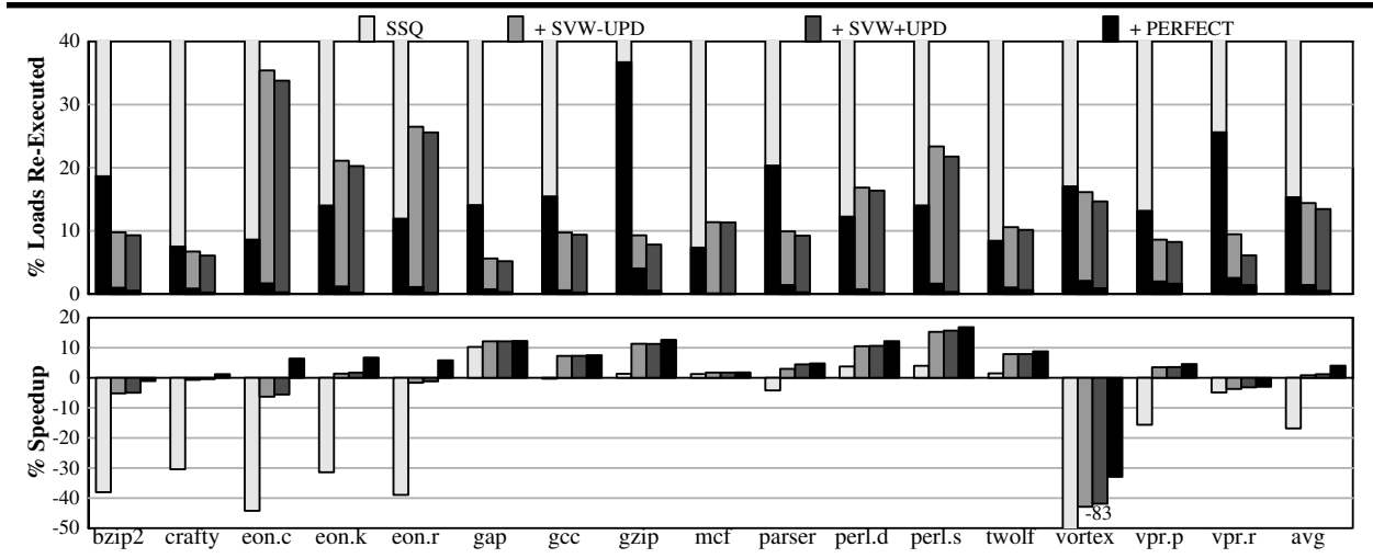
FIGURE 6. SSQ re-execution rate (top) and performance (bottom).
