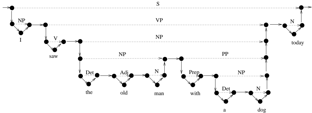
Fig. 4. Parsed sentence as a nested word
