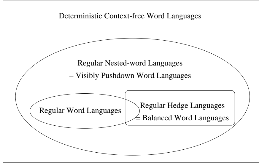
Fig. 12. Relationship among languages classes
