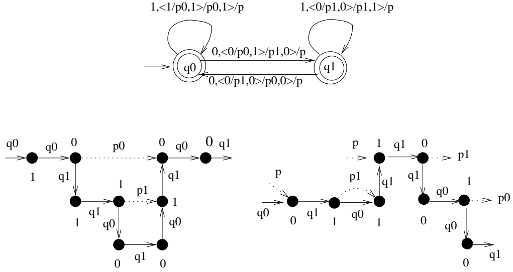
Fig. 6. Example of an NWA and its runs
