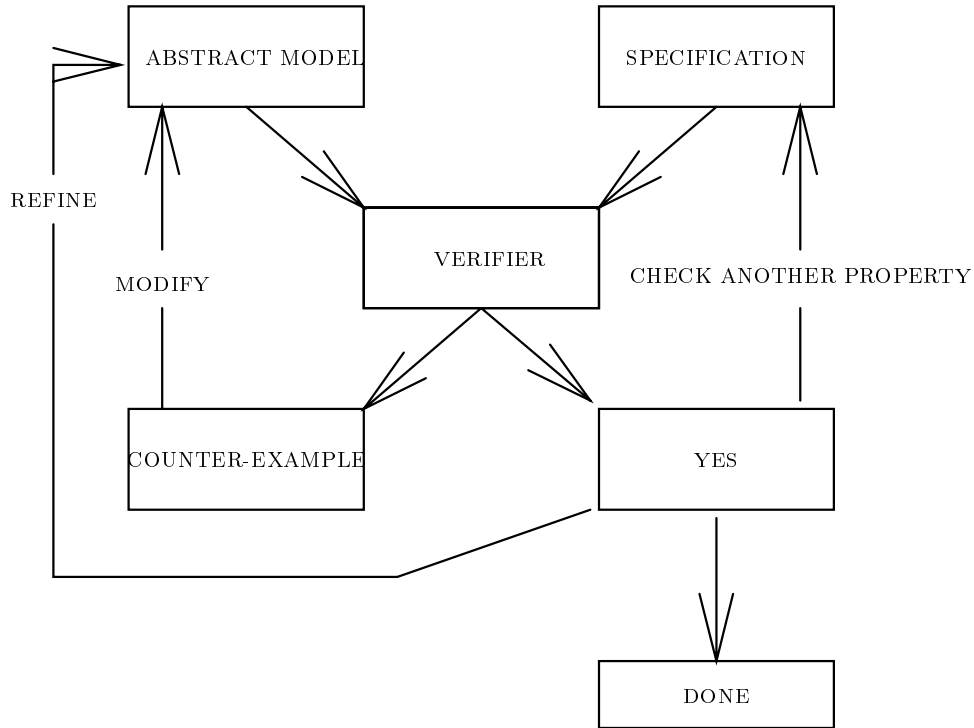
Figure 1: Model checking methodology
