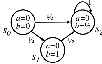
Fig. 13. A multi-valued Kripke structure \mathcal{M} where the atomic propositions and the transition relation take truth values over the quasi-Boolean algebra \mathfrak{B}_3 .
