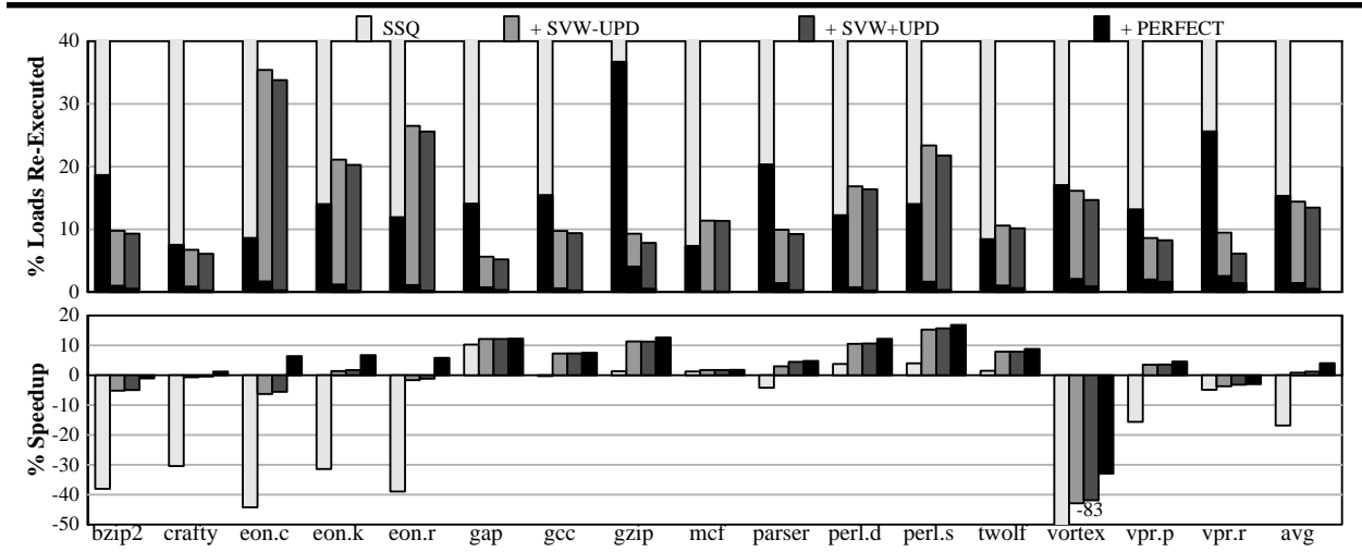
FIGURE 6. SSQ re-execution rate (top) and performance (bottom).
