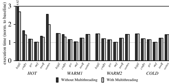
Figure 8. DISE overhead with multithreading.
