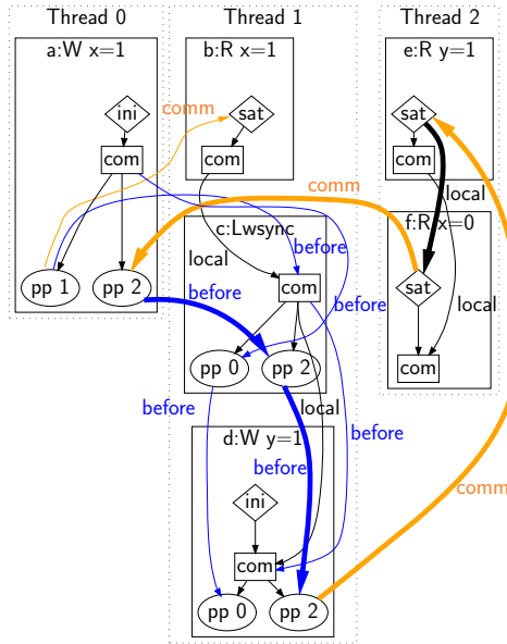
Test WRC+lwsync+addr Candidate 4
