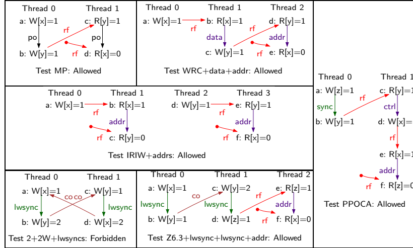
Fig. 1. Examples illustrating the POWER memory model
