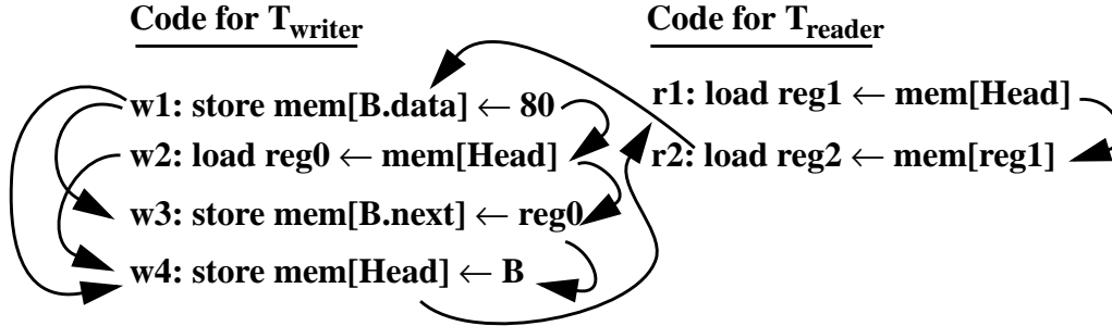
Figure 2. Value Prediction with Simple Verification Violating SC. The example execution of Figure 1(d) forms a cycle, violating SC.
