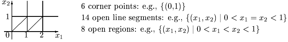
FIGURE 3. Equivalence classes of planar region equivalence
