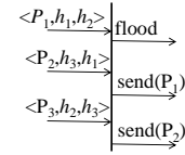
Figure 1: A scenario describing the learning switch. In the scenario, a packet is denoted by a 3-tuple: \langle incoming port, source MAC, destination MAC \rangle .
