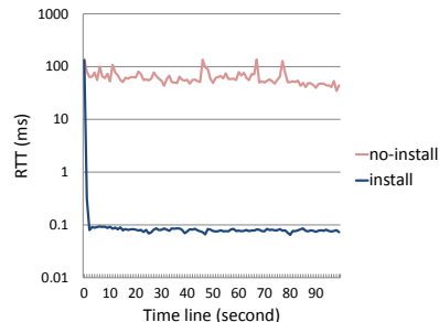
Figure 15: Effects of flow table rule installation.
